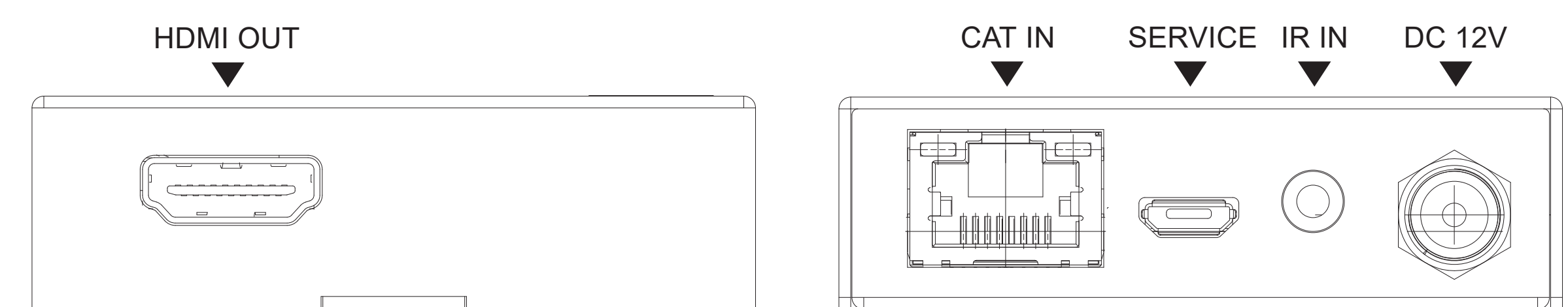
Receiver
