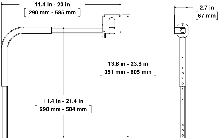
STB-10PVMGUX-W GONDOLA UPRIGHT MOUNT
