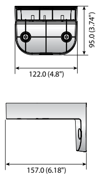
SBP-300WM0/120WM
