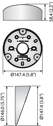
SBP-300TM1
