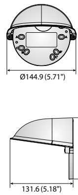
SBV-120WC
