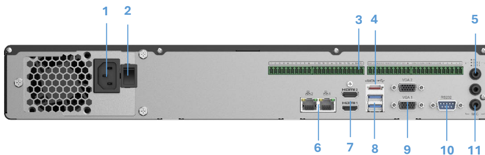
Back Panel
