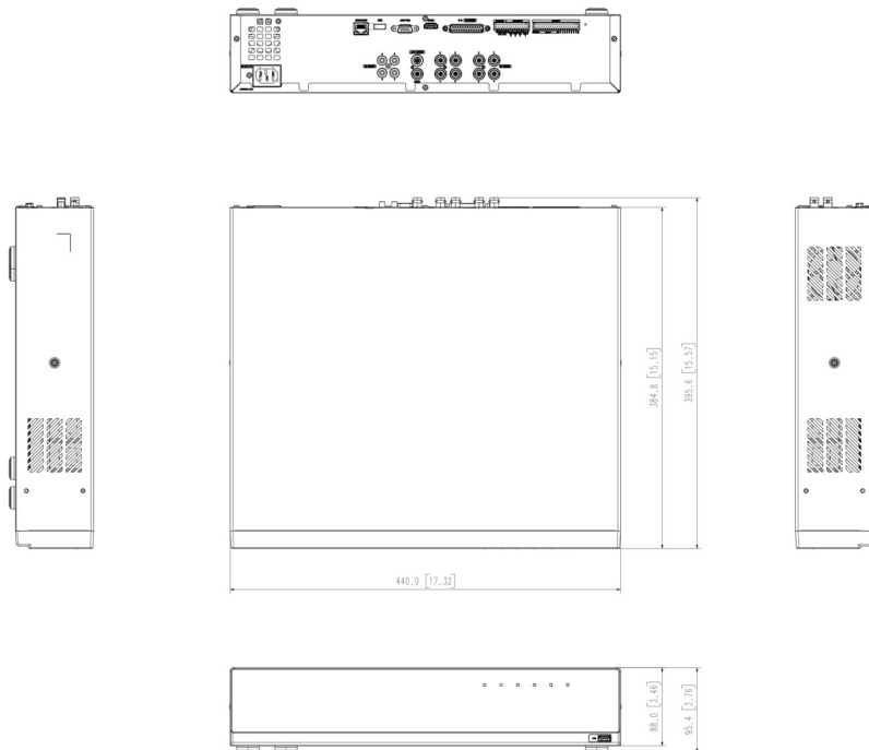
Appearance drawing HRX-835A, HRX-835/TE Unit : mm [inches]
