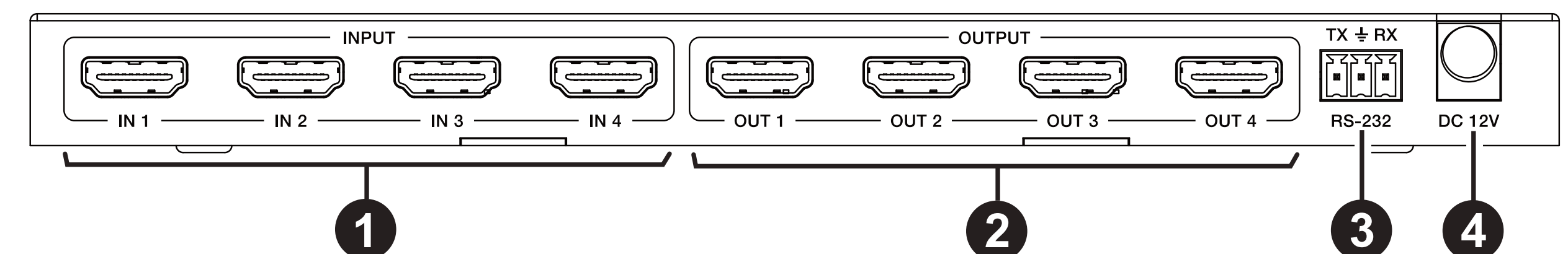
Rear Panel
