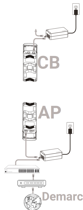
Figure 2: AP to CB Topology
